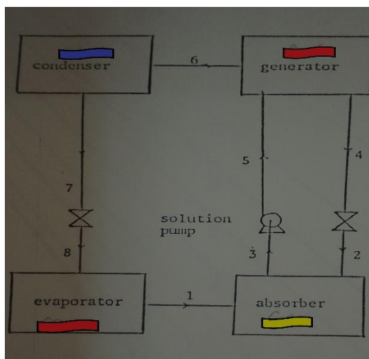
Figure 7. Heat pump diagram
